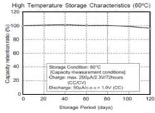
High Temperature Storage Characteristics (60°C)
