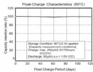
Float-Charge Characteristics (60°C)
