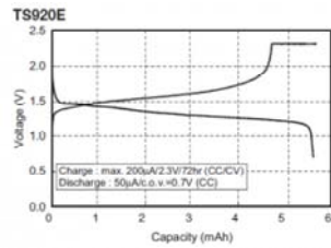
Charge/Discharge Characteristics
